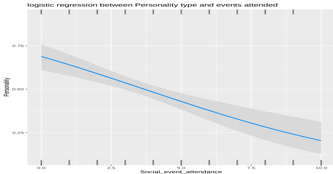
Figure 11 Logistic regression graph for introvert group and social event attendance
