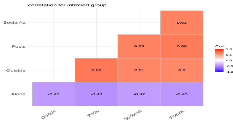
Figure 6 Correlation matrix for introvert group
