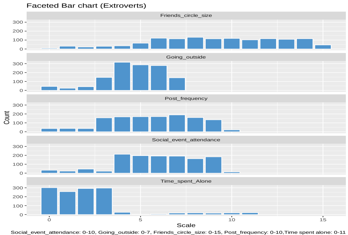
Figure 3 Faceted bar graph of variables grouped for extroverts.
