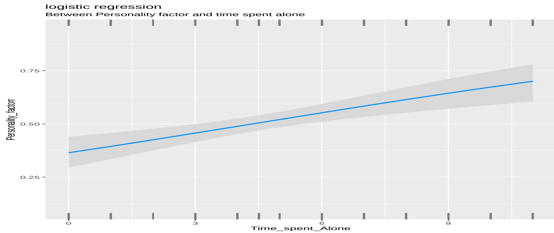
Figure 13 Logistic regression with imputed data for introvert group and time spent alone
