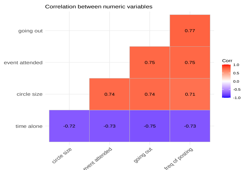
Figure 5 Correlation matrix for numeric variables
