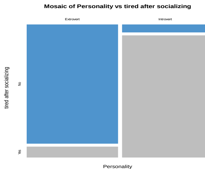
Figure 8 Mosaic plot of personality type and feeling tired after socializing.
