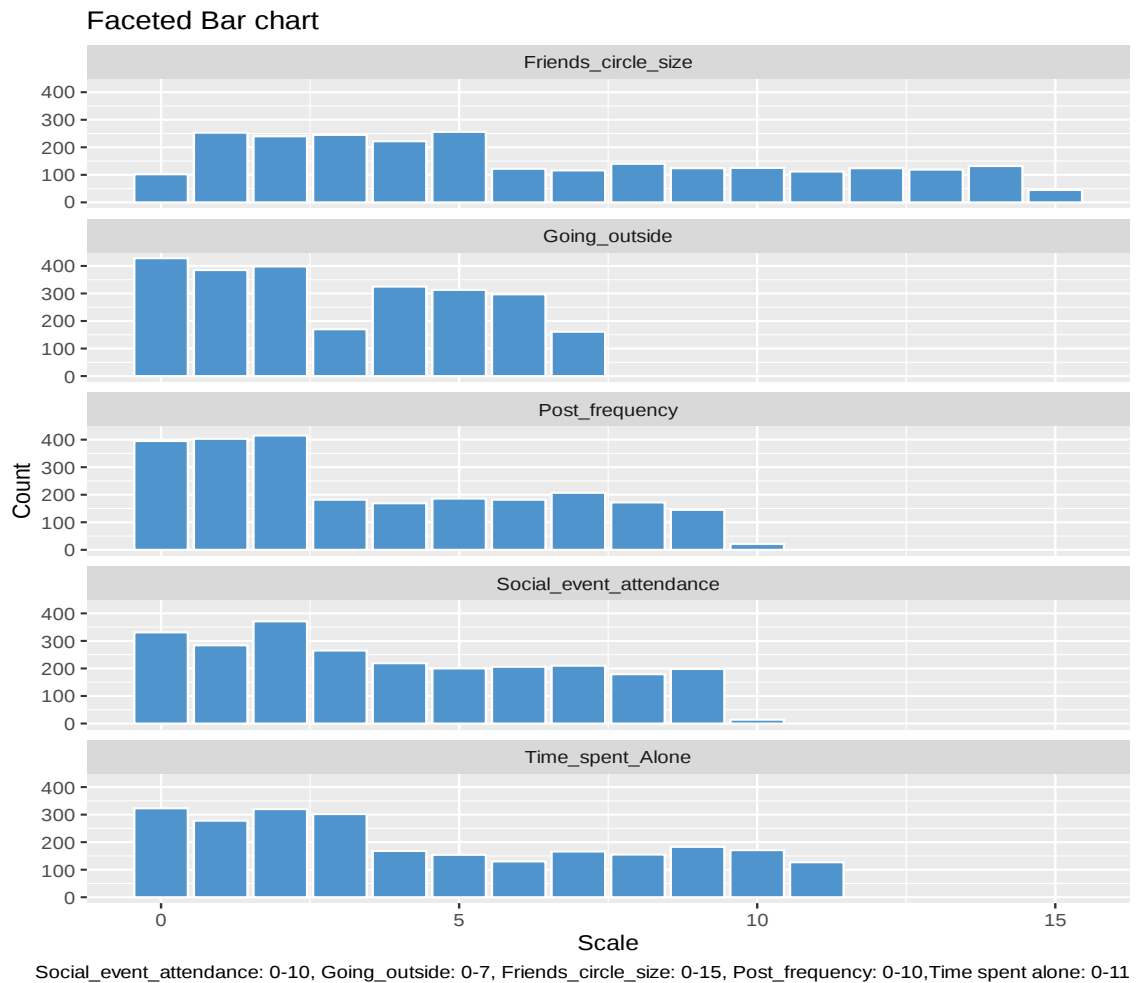
Figure 1 Faceted bar graph of discrete variables
