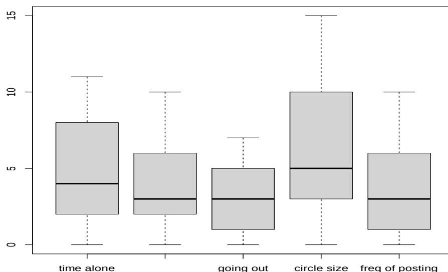
Figure 4 Boxplot of numeric variables
