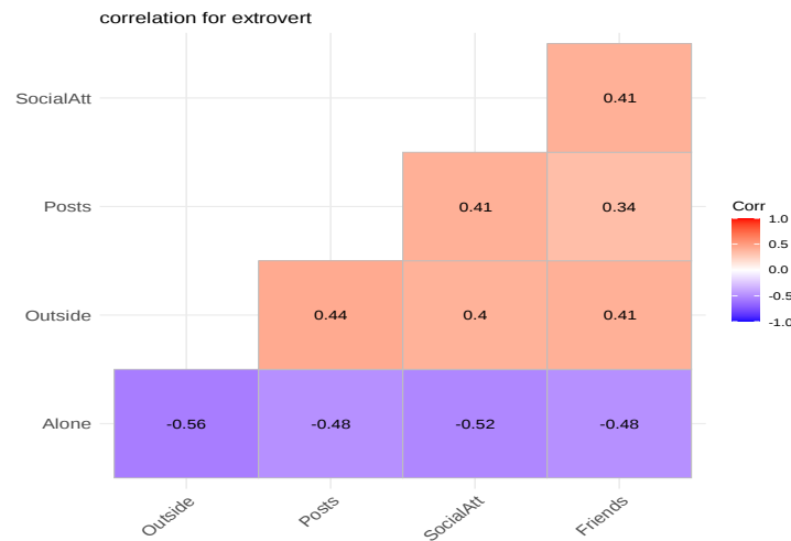
Figure 7 Correlation matrix for extrovert group
