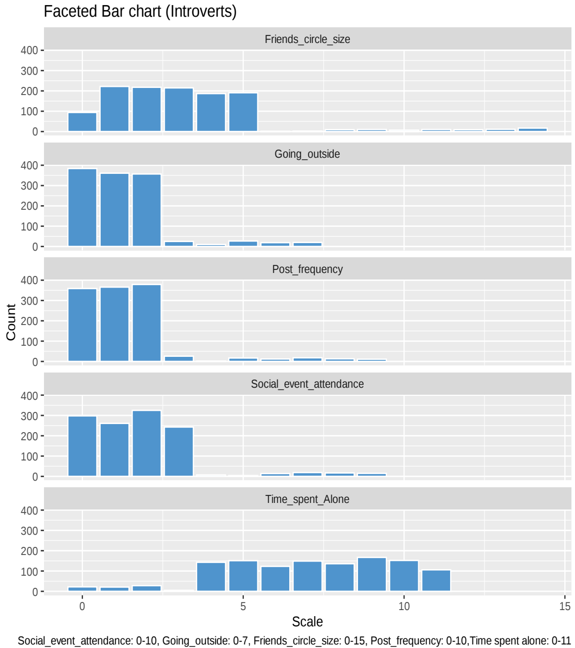
Figure 2 Faceted bar graph of variables grouped for introverts.
